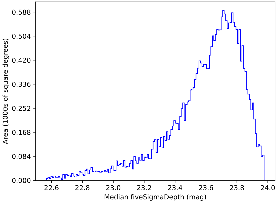
too_elab_r16_d2_giz_v3.4_10yrs Yr 1 i band: Median fiveSigmaDepth
