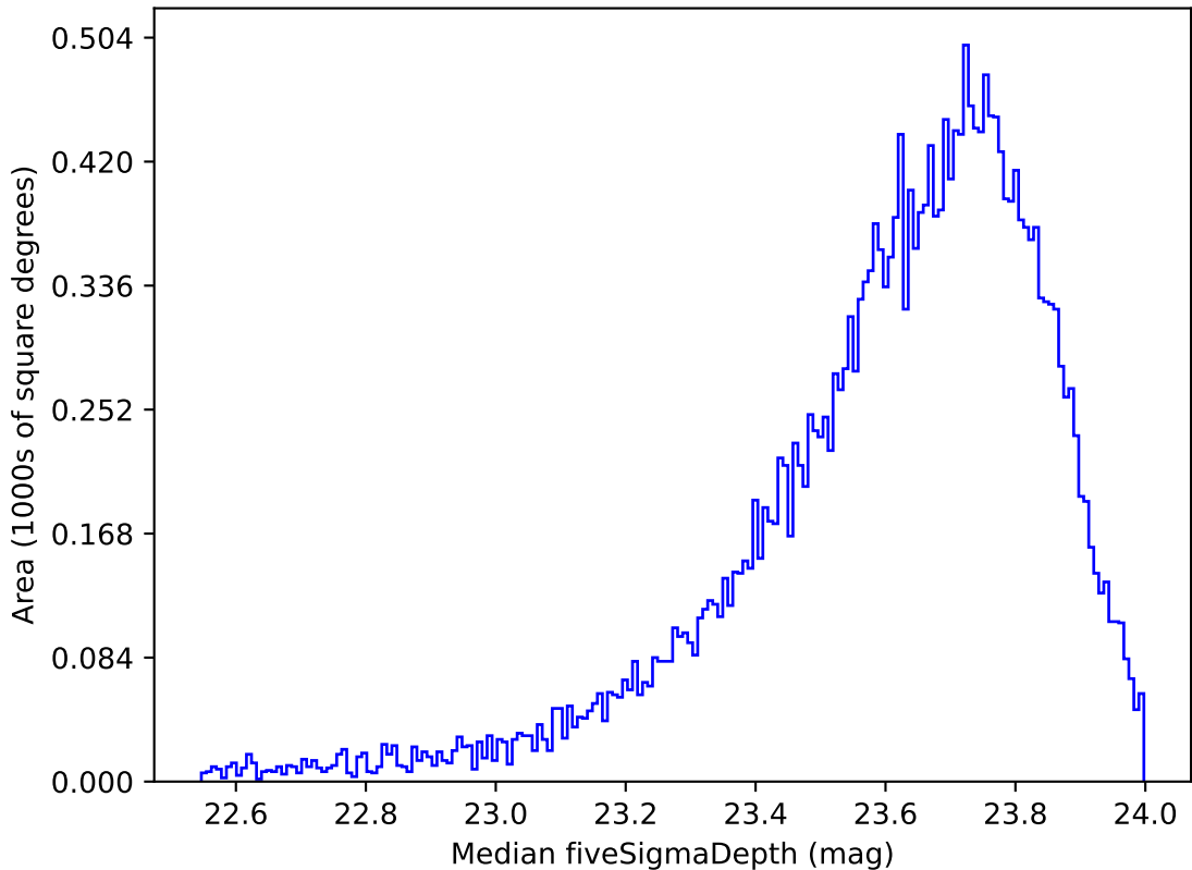
too_elab_r16_d2_giz_v3.4_10yrs Yr 1 i band: Median fiveSigmaDepth
