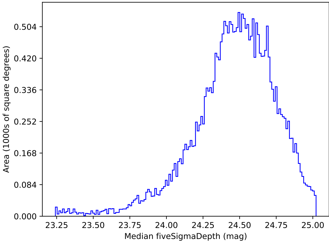
too_elab_r16_d2_giz_v3.4_10yrs Yr 1 g band: Median fiveSigmaDepth
