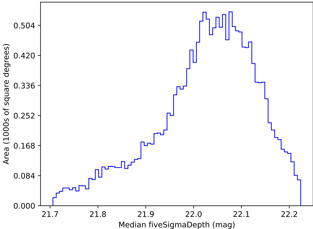
too_elab_r16_d2_giz_v3.4_10yrs WFD y band: Median fiveSigmaDepth
