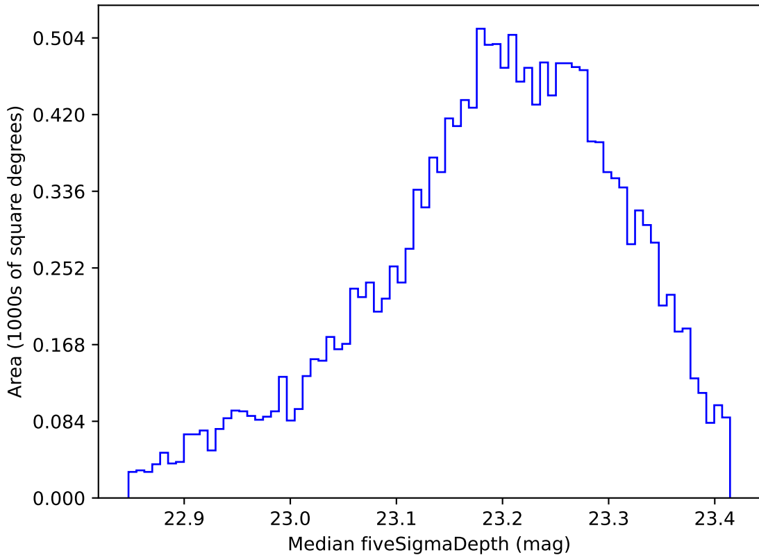
too_elab_r16_d2_giz_v3.4_10yrs WFD u band: Median fiveSigmaDepth
