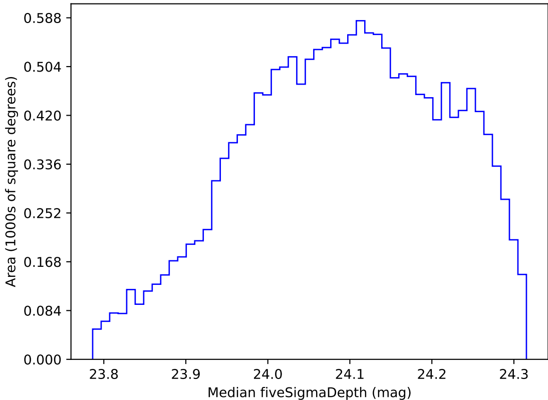
too_elab_r16_d2_giz_v3.4_10yrs WFD r band: Median fiveSigmaDepth
