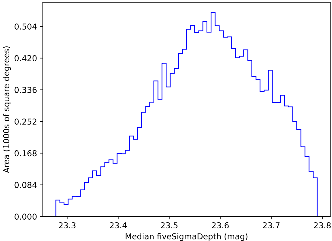
too_elab_r16_d2_giz_v3.4_10yrs WFD i band: Median fiveSigmaDepth
