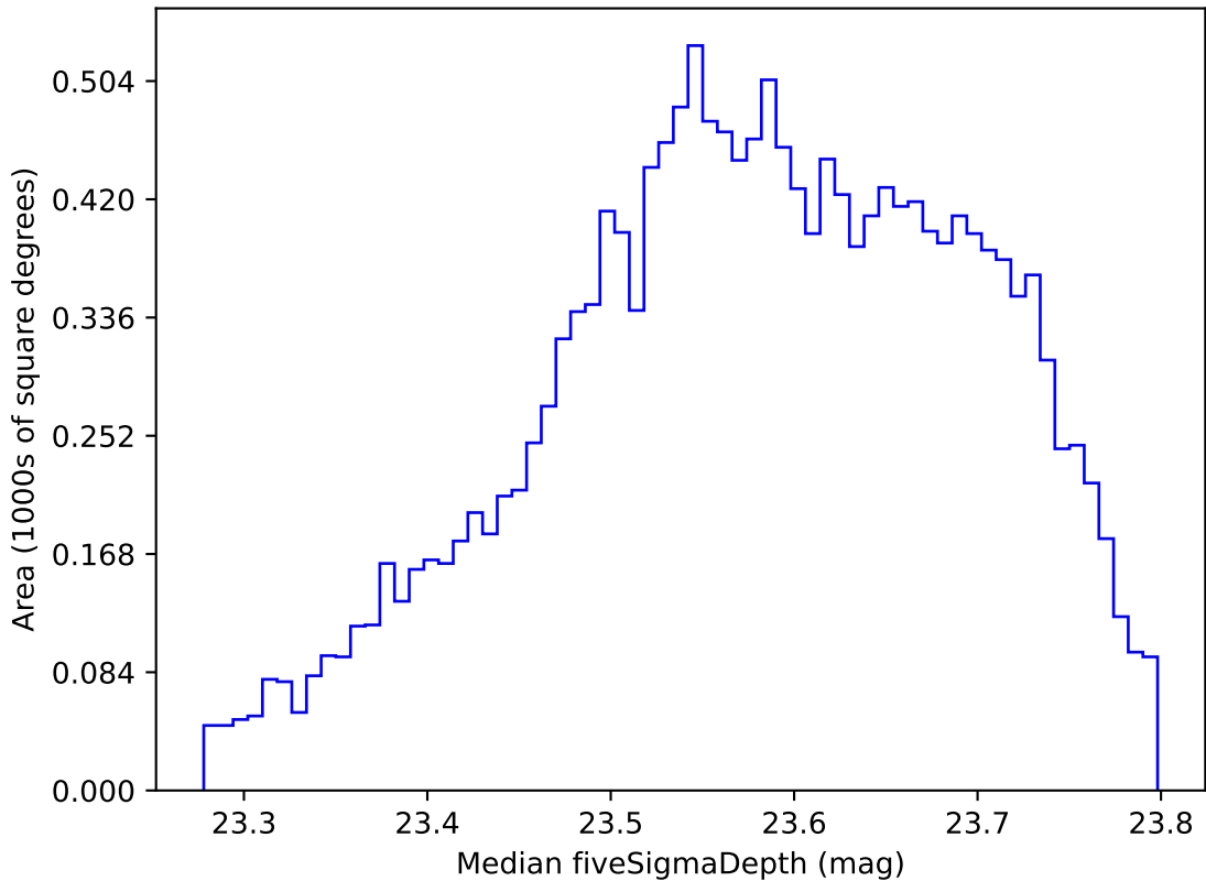
too_elab_r16_d2_giz_v3.4_10yrs WFD i band: Median fiveSigmaDepth
