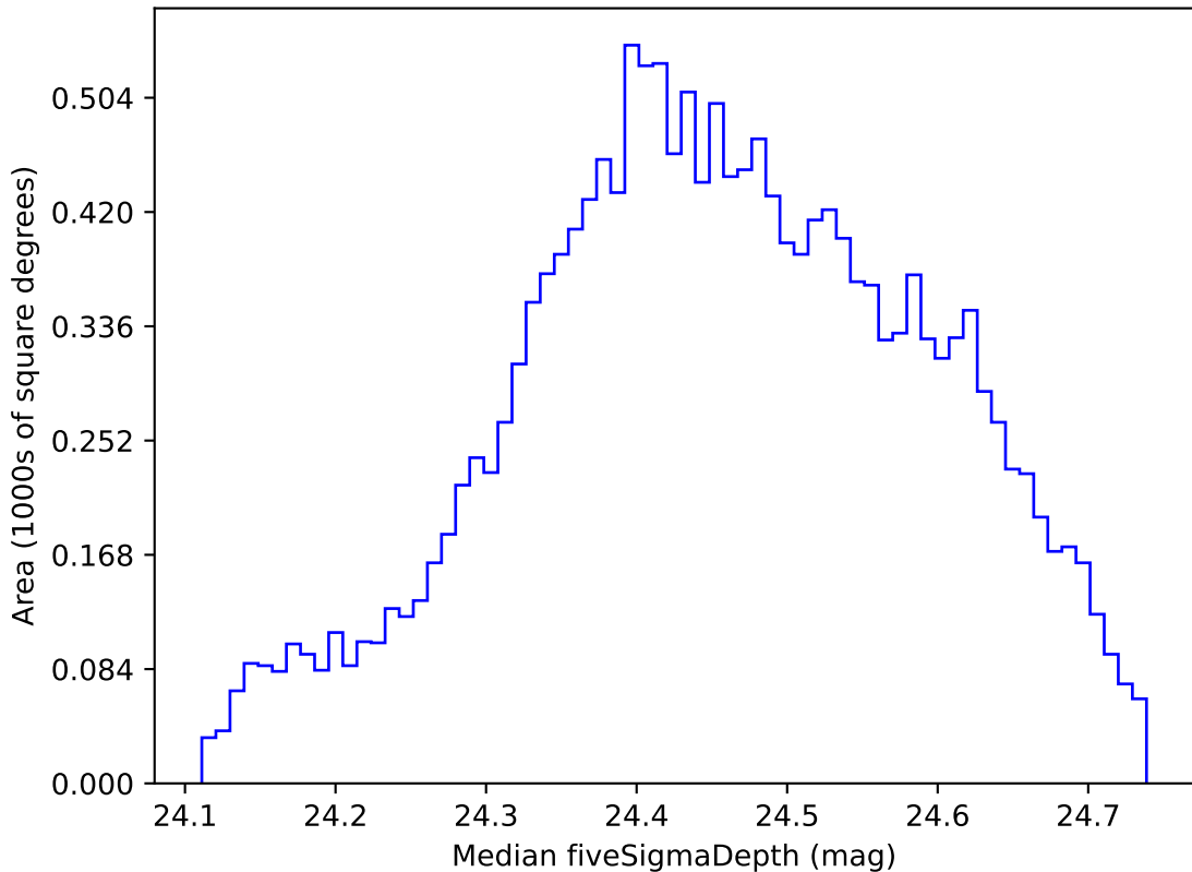
too_elab_r16_d2_giz_v3.4_10yrs WFD g band: Median fiveSigmaDepth
