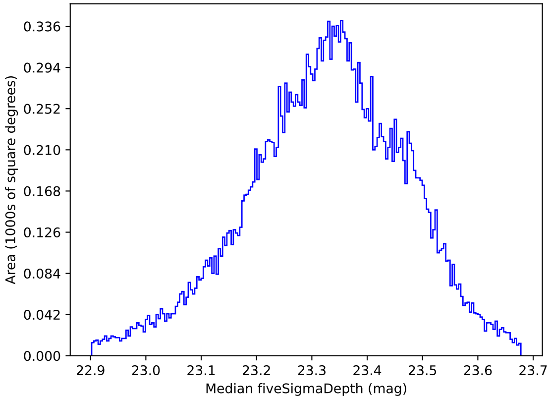
too_elab_r16_d2_giz_v3.4_10yrs All sky all bands: Median fiveSigmaDepth
