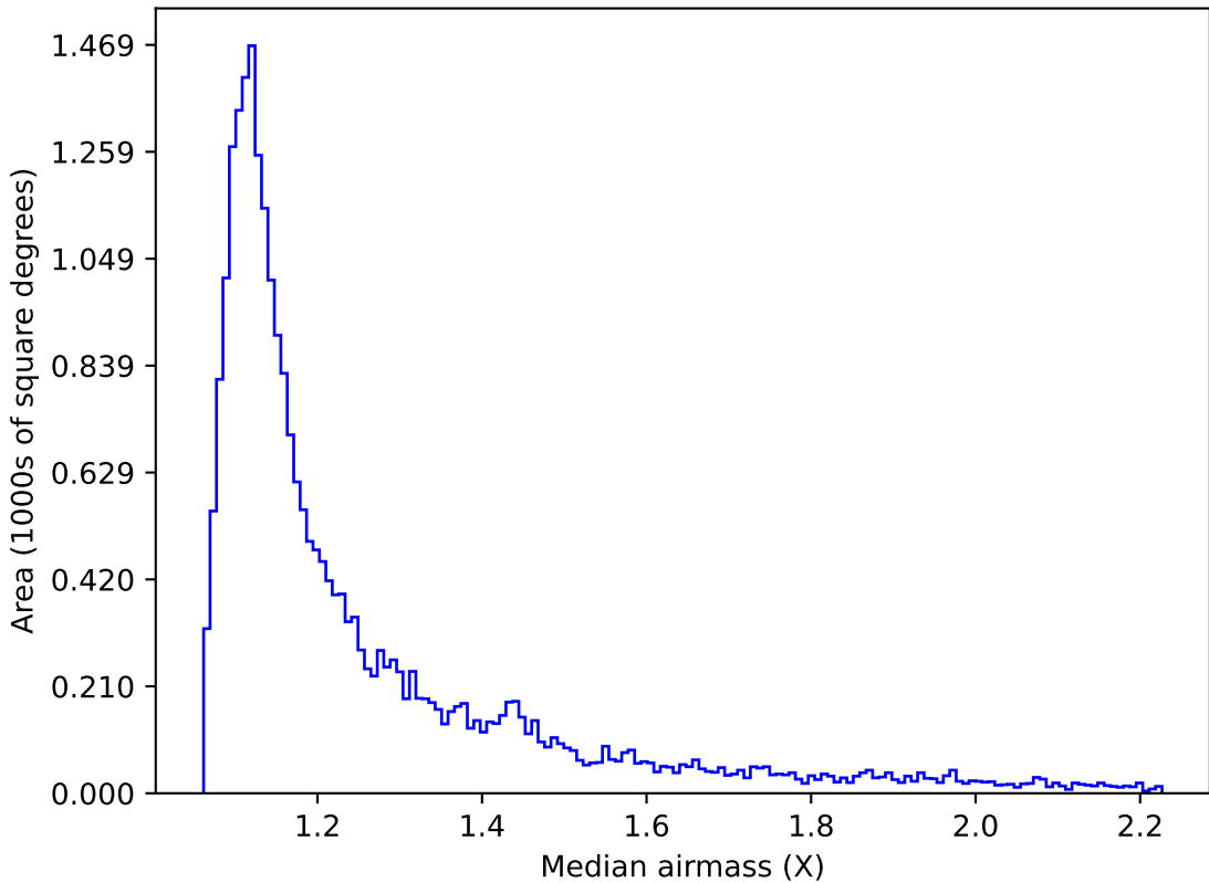
too_elab_r16_d2_giz_v3.4_10yrs Yr 1 z band: Median airmass
