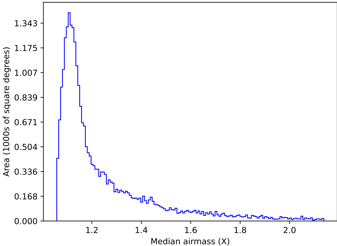
too_elab_r16_d2_giz_v3.4_10yrs Yr 1 r band: Median airmass
