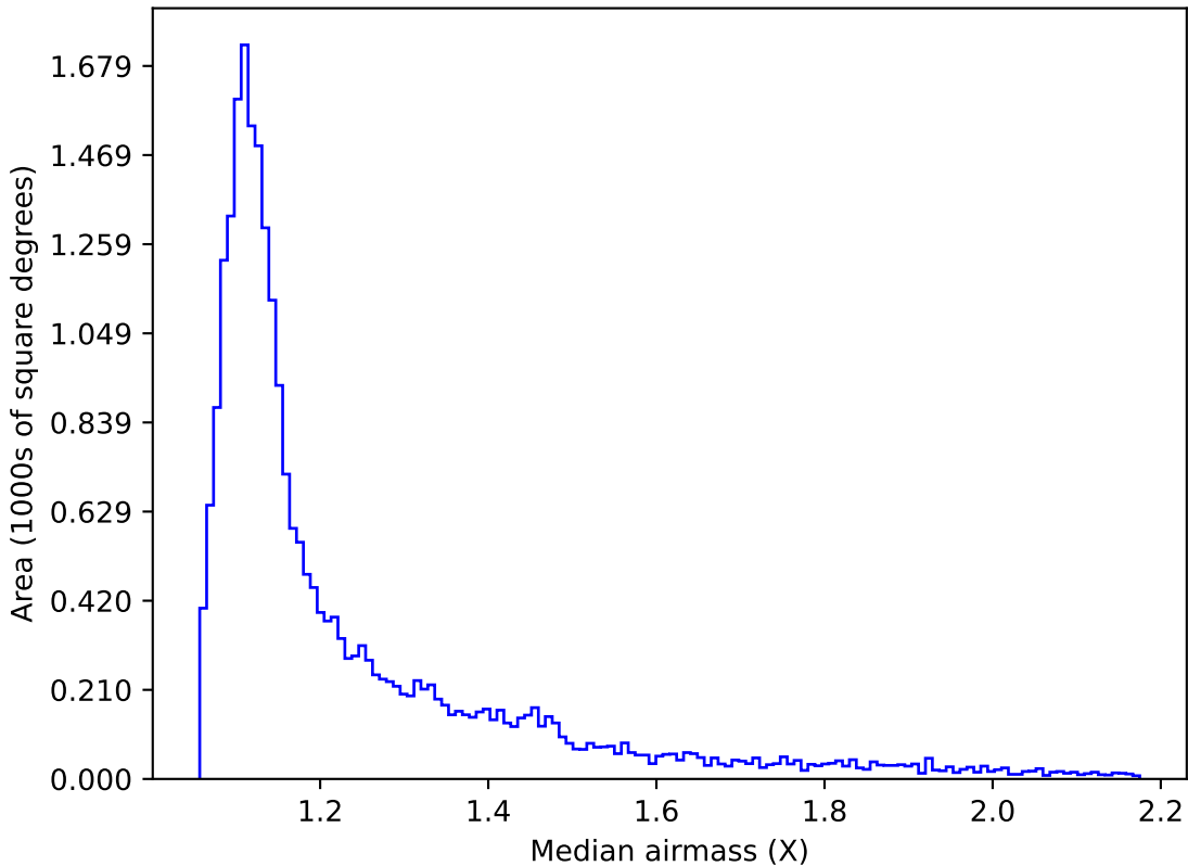
too_elab_r16_d2_giz_v3.4_10yrs Yr 1 i band: Median airmass
