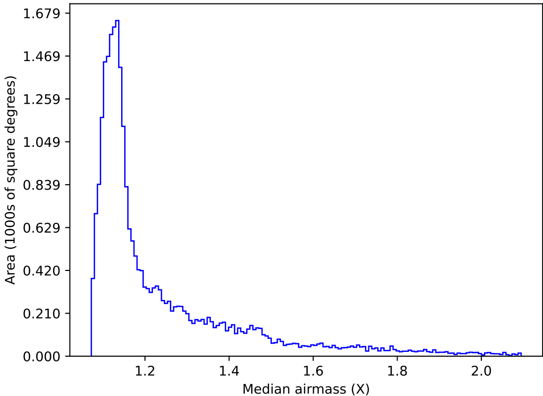
too_elab_r16_d2_giz_v3.4_10yrs Yr 1 all bands: Median airmass
