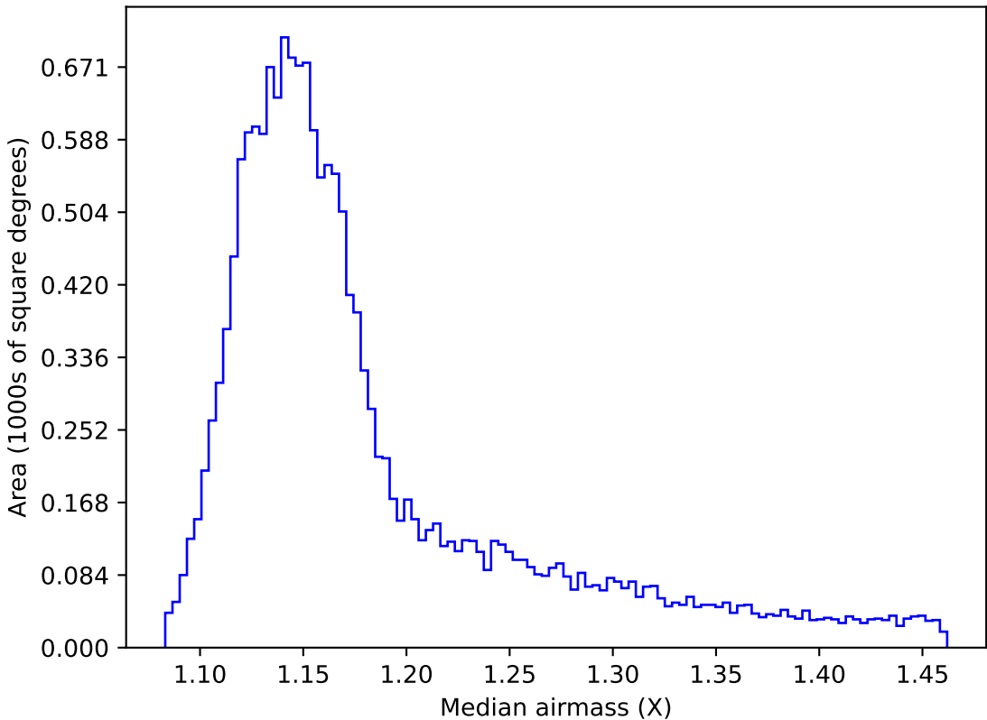
too_elab_r16_d2_giz_v3.4_10yrs WFD z band: Median airmass
