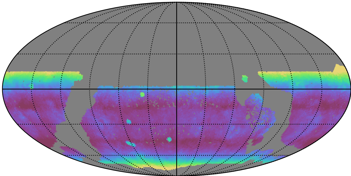
too_elab_r16_d2_giz_v3.4_10yrs WFD y band: Median airmass
