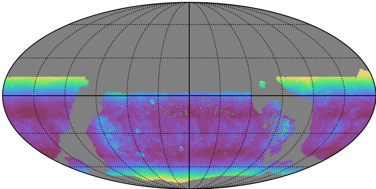
too_elab_r16_d2_giz_v3.4_10yrs WFD u band: Median airmass
