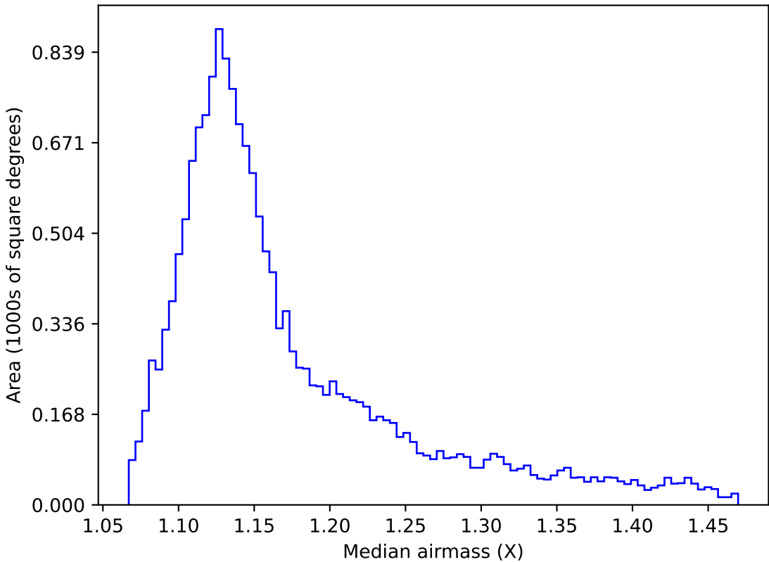
too_elab_r16_d2_giz_v3.4_10yrs WFD u band: Median airmass
