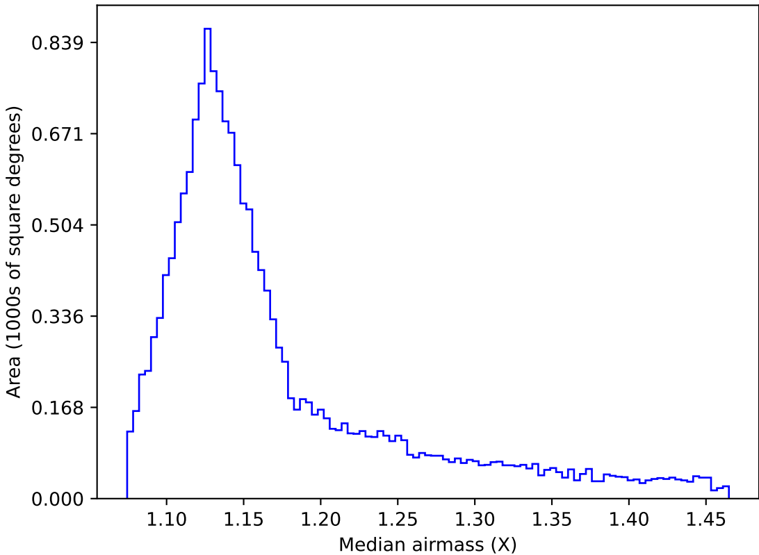
too_elab_r16_d2_giz_v3.4_10yrs WFD r band: Median airmass
