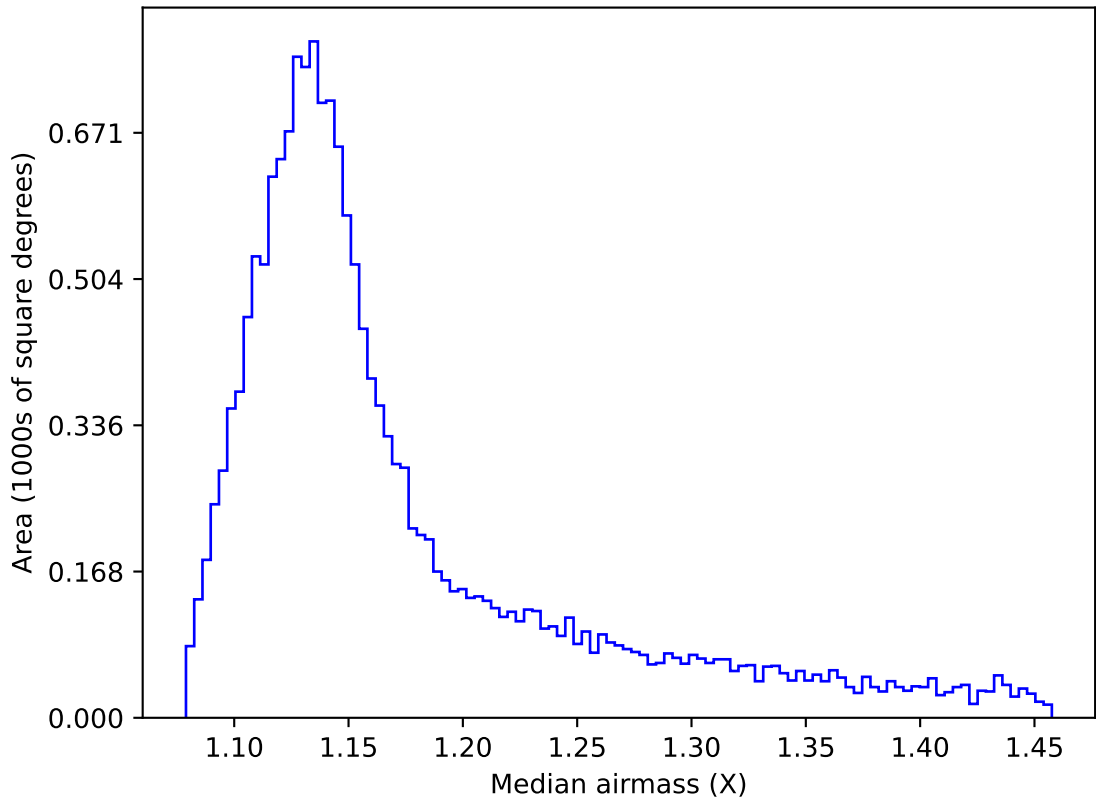
too_elab_r16_d2_giz_v3.4_10yrs WFD i band: Median airmass
