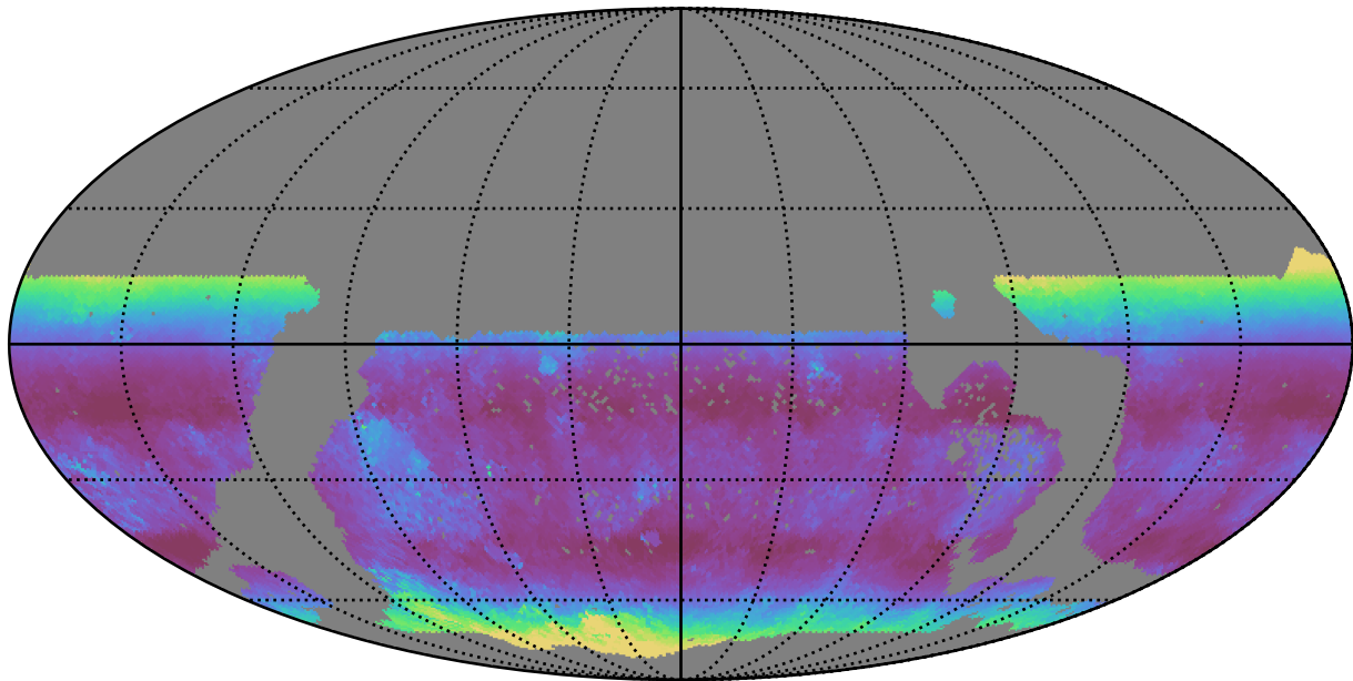
too_elab_r16_d2_giz_v3.4_10yrs WFD g band: Median airmass
