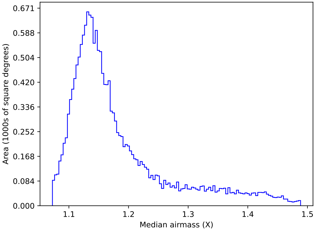
too_elab_r16_d2_giz_v3.4_10yrs WFD g band: Median airmass
