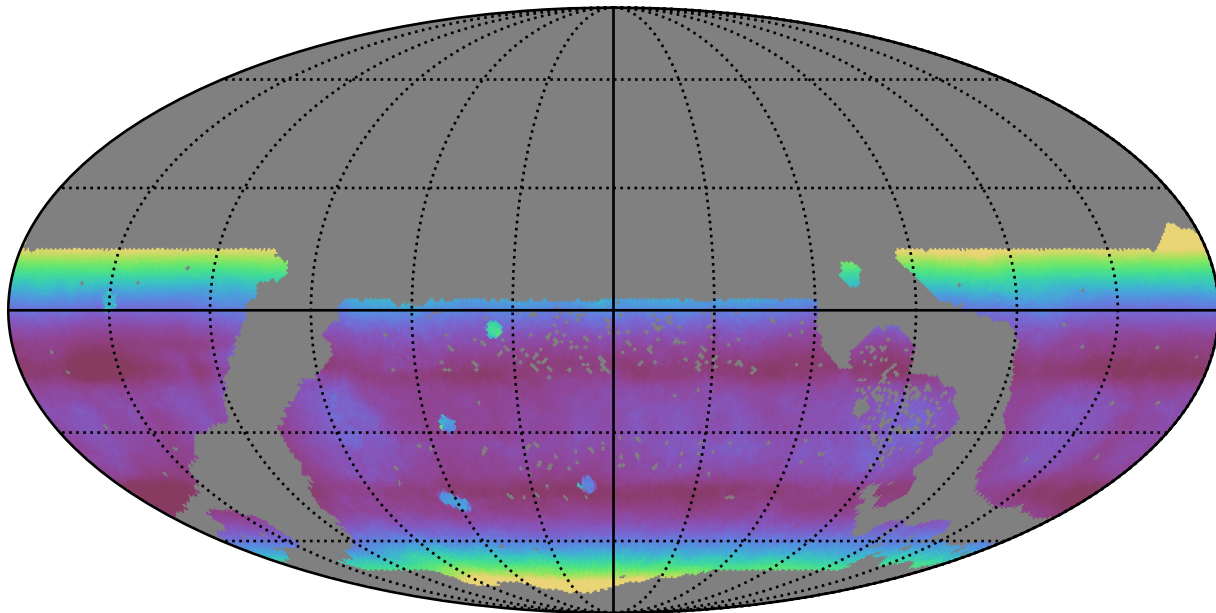
too_elab_r16_d2_giz_v3.4_10yrs WFD all bands: Median airmass
