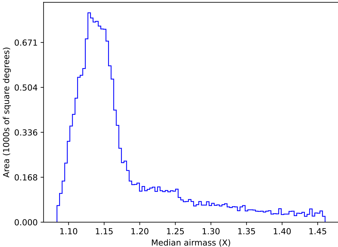
too_elab_r16_d2_giz_v3.4_10yrs WFD all bands: Median airmass
