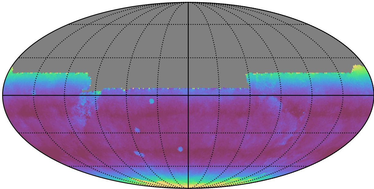
too_elab_r16_d2_giz_v3.4_10yrs All sky y band: Median airmass
