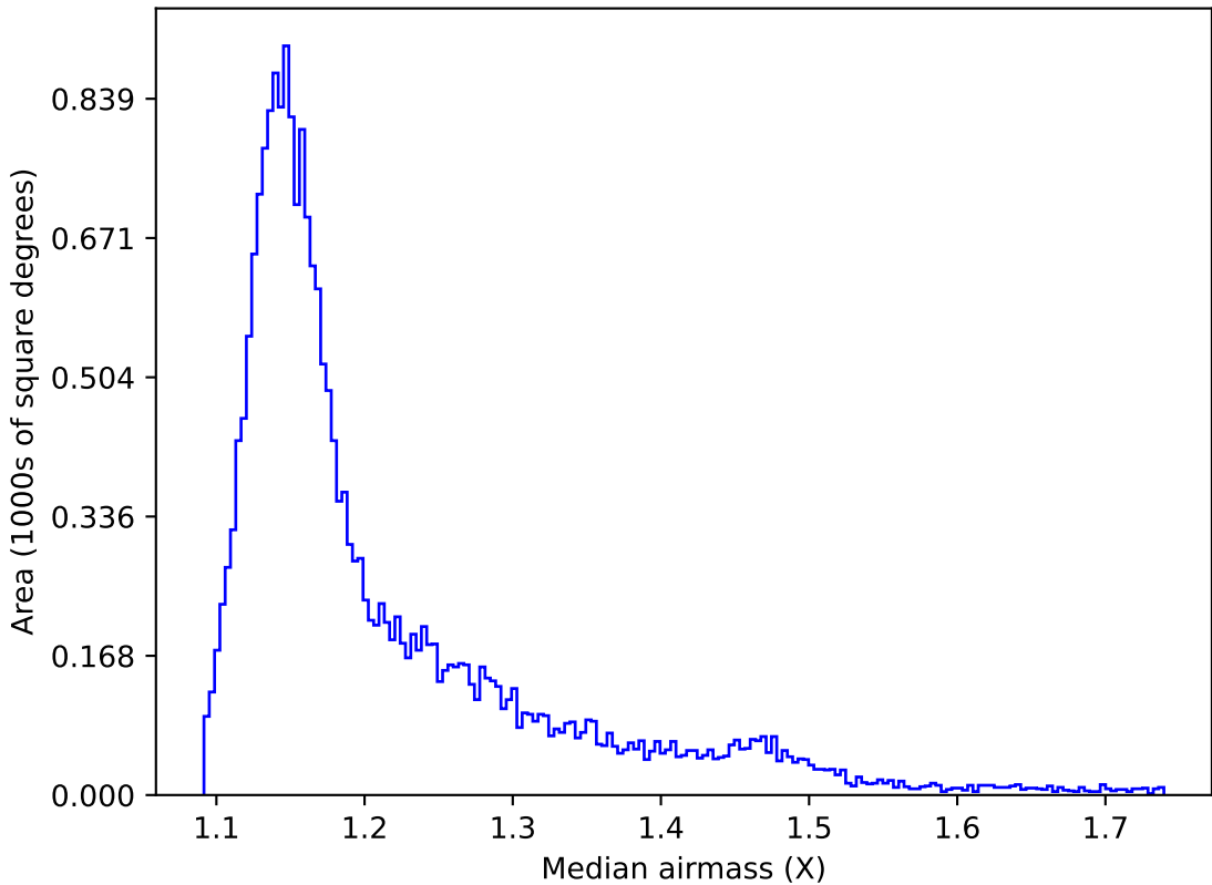
too_elab_r16_d2_giz_v3.4_10yrs All sky y band: Median airmass
