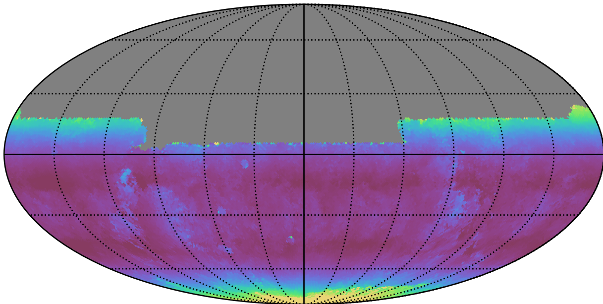
too_elab_r16_d2_giz_v3.4_10yrs All sky u band: Median airmass
