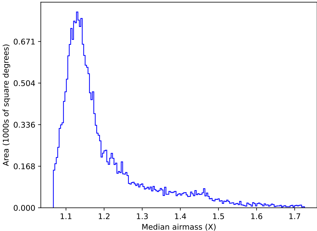
too_elab_r16_d2_giz_v3.4_10yrs All sky u band: Median airmass
