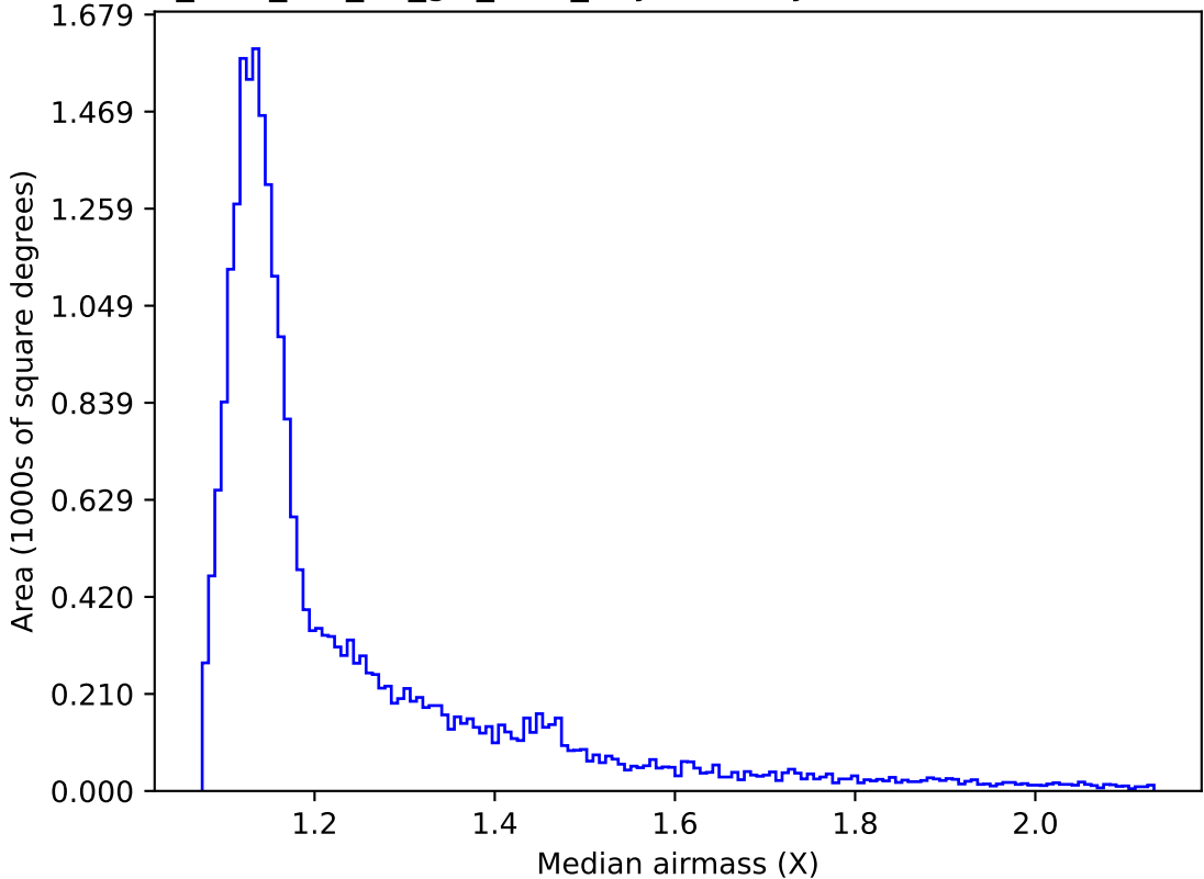
too_elab_r16_d2_giz_v3.4_10yrs All sky r band: Median airmass
