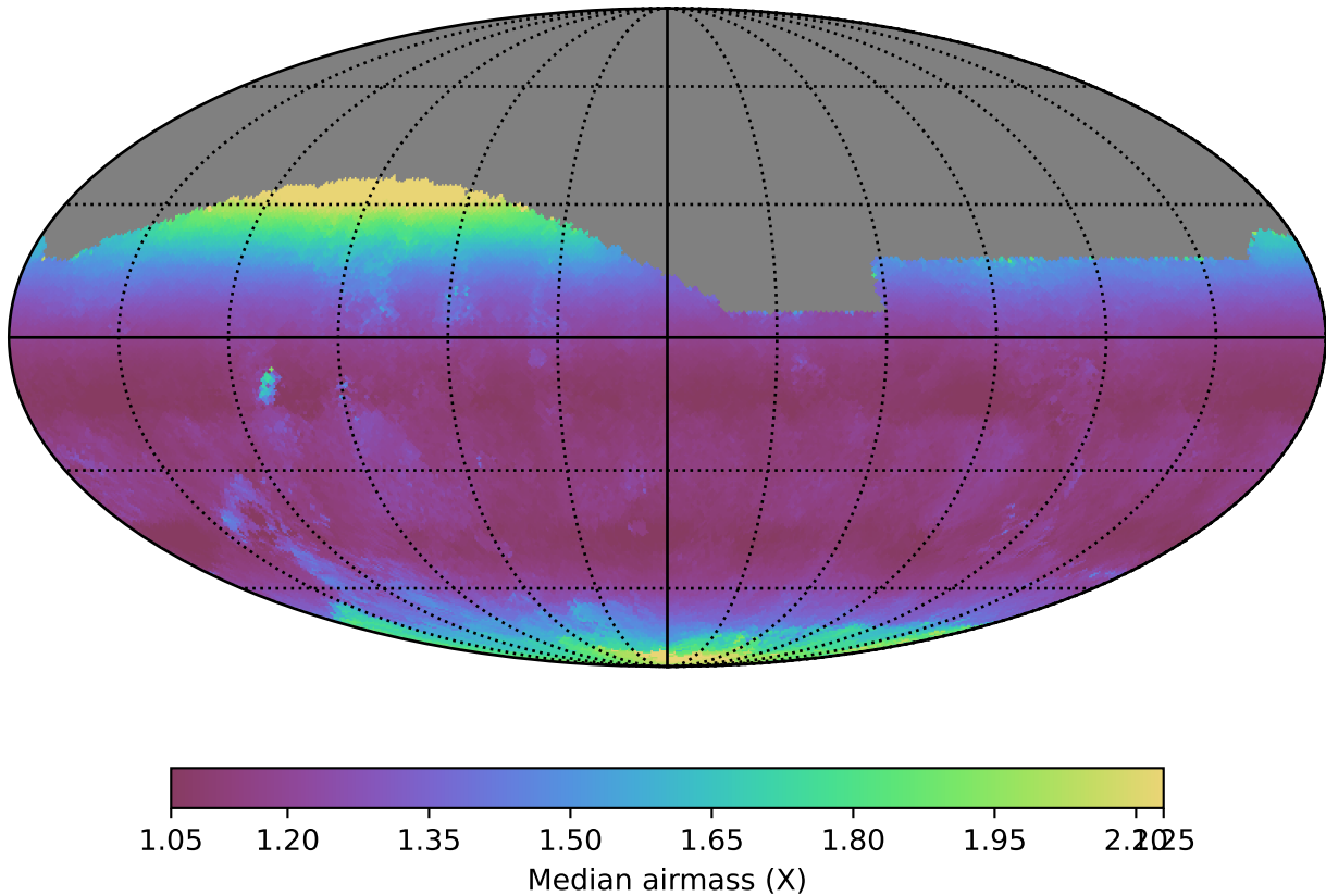
too_elab_r16_d2_giz_v3.4_10yrs All sky g band: Median airmass
