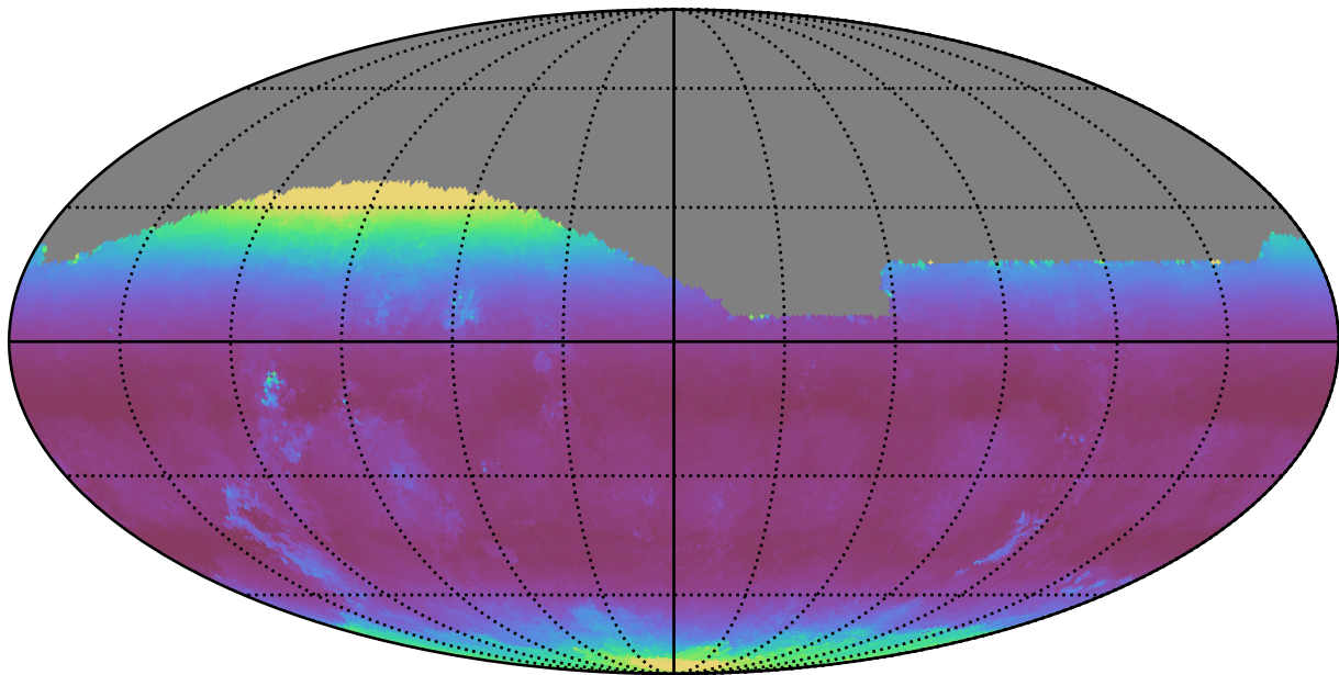
too_elab_r16_d2_giz_v3.4_10yrs All sky g band: Median airmass
