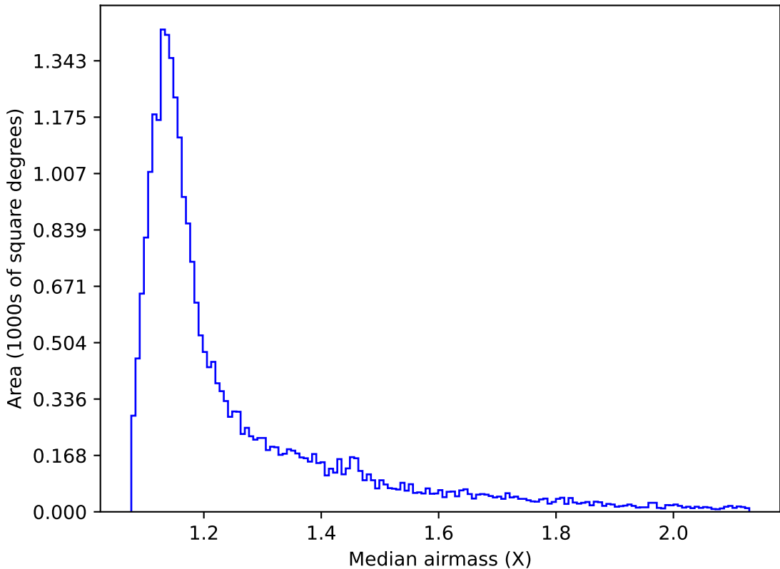
too_elab_r16_d2_giz_v3.4_10yrs All sky g band: Median airmass
