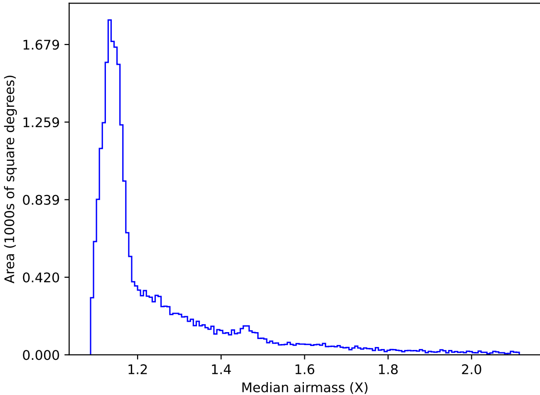
too_elab_r16_d2_giz_v3.4_10yrs All sky all bands: Median airmass
