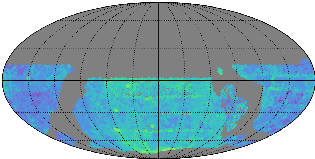
too_elab_r16_d2_giz_v3.4_10yrs WFD y band: Median Season Length
