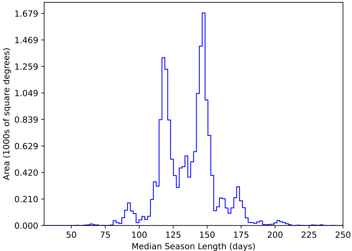
too_elab_r16_d2_giz_v3.4_10yrs WFD y band: Median Season Length
