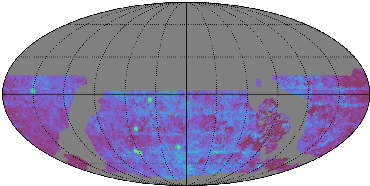
too_elab_r16_d2_giz_v3.4_10yrs WFD u band: Median Season Length
