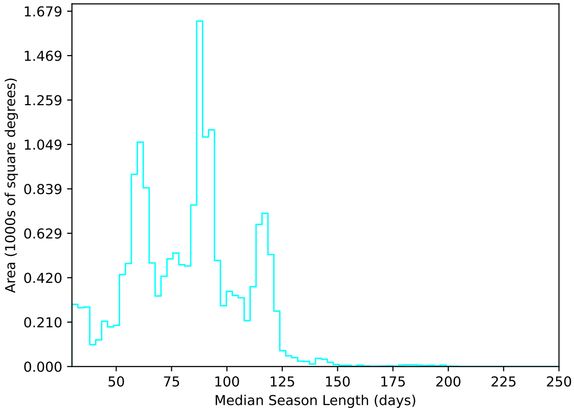
too_elab_r16_d2_giz_v3.4_10yrs WFD u band: Median Season Length
