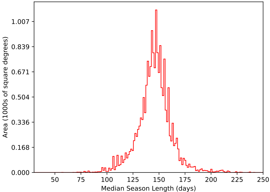
too_elab_r16_d2_giz_v3.4_10yrs WFD i band: Median Season Length
