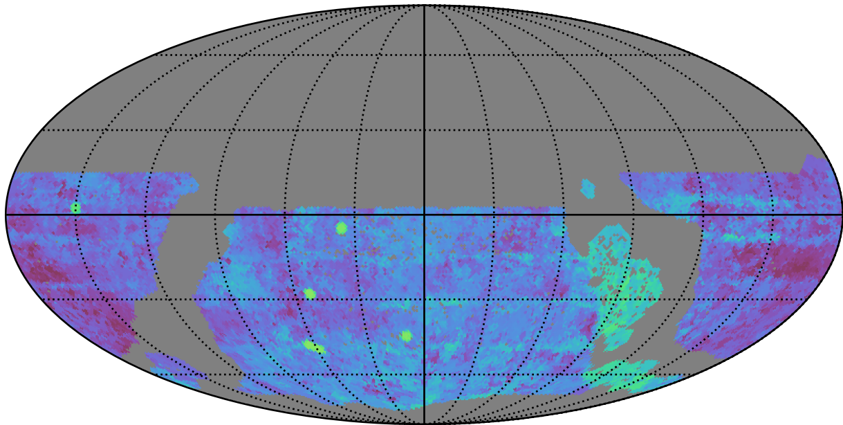
too_elab_r16_d2_giz_v3.4_10yrs WFD g band: Median Season Length
