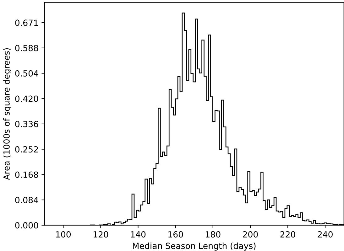
too_elab_r16_d2_giz_v3.4_10yrs WFD all bands: Median Season Length
