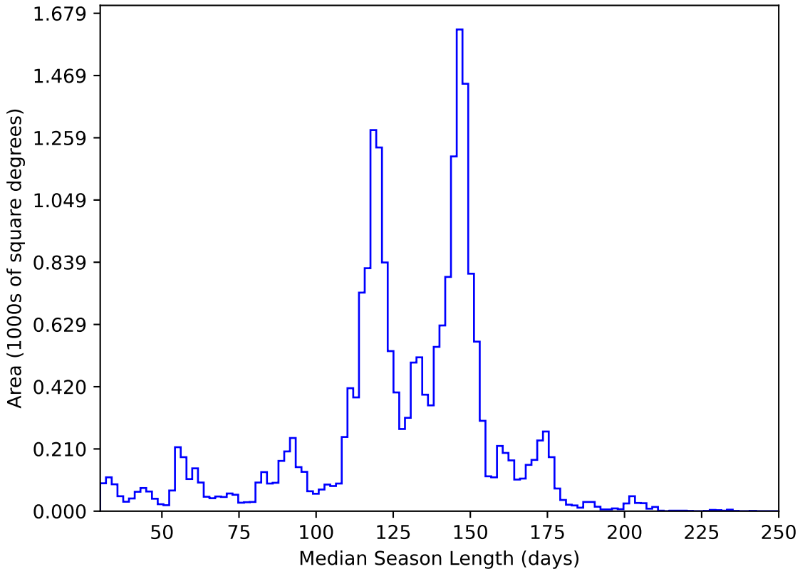
too_elab_r16_d2_giz_v3.4_10yrs All sky y band: Median Season Length
