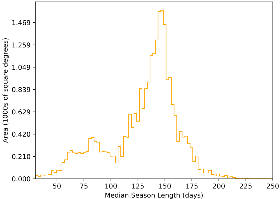
too_elab_r16_d2_giz_v3.4_10yrs All sky r band: Median Season Length
