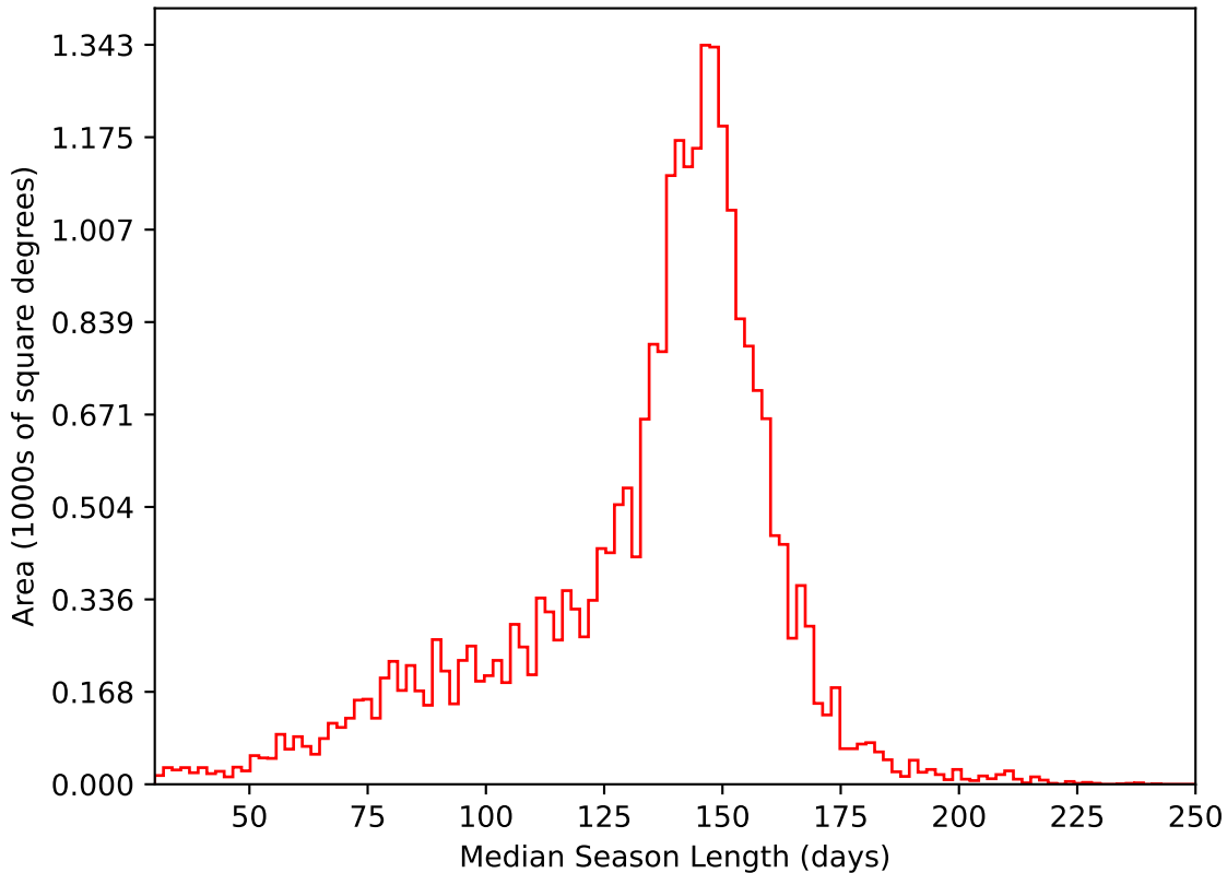
too_elab_r16_d2_giz_v3.4_10yrs All sky i band: Median Season Length
