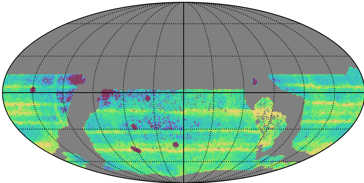
too_elab_r16_d2_giz_v3.4_10yrs WFD: Median Intra-Night Gap
