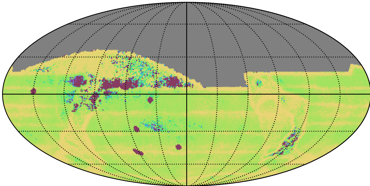
too_elab_r16_d2_giz_v3.4_10yrs All sky: Median Intra-Night Gap
