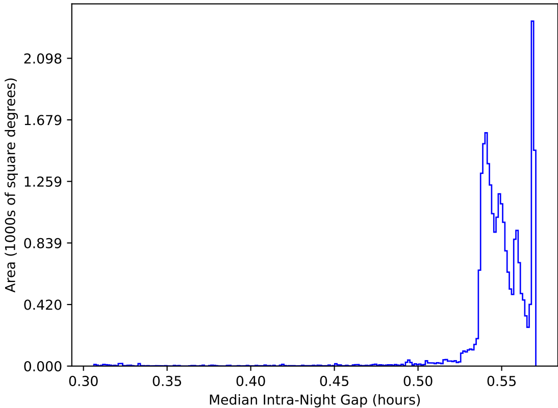
too_elab_r16_d2_giz_v3.4_10yrs All sky: Median Intra-Night Gap
