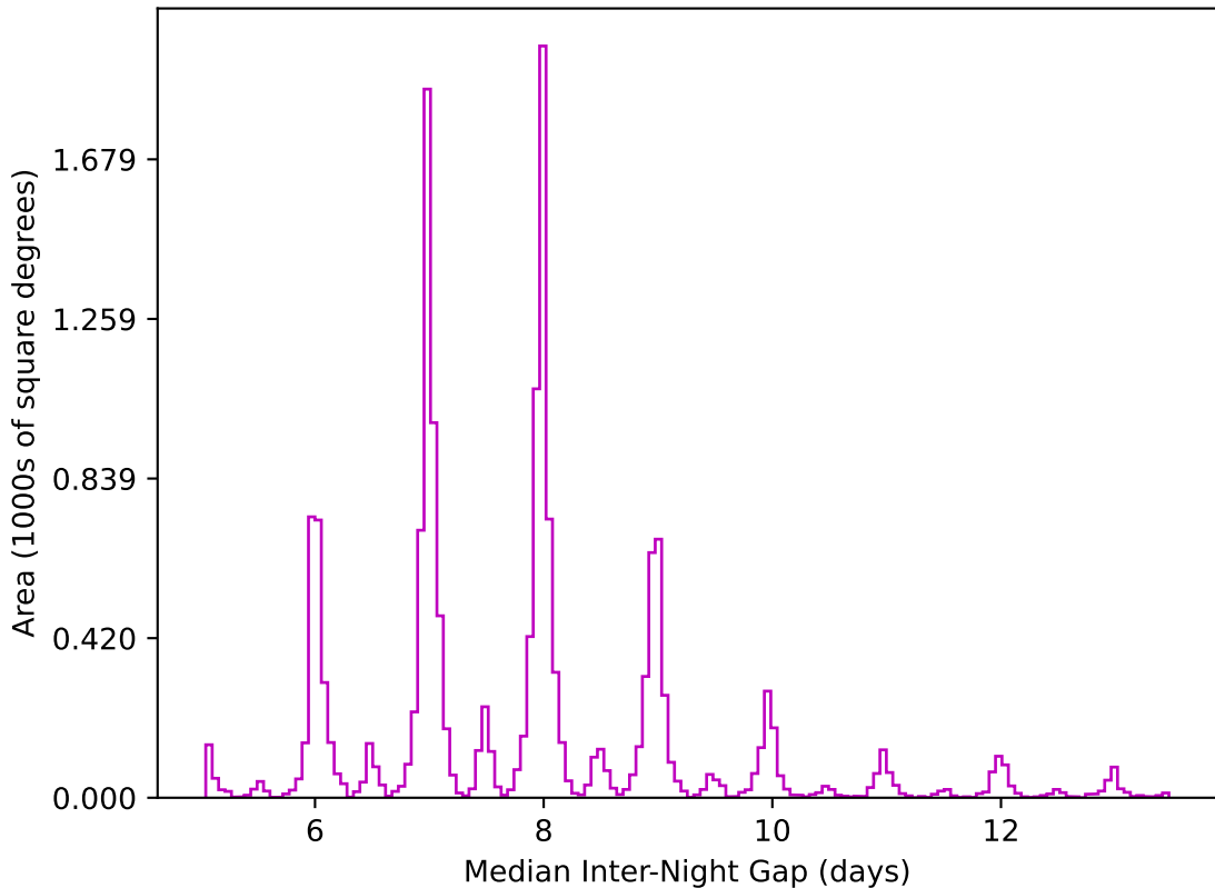
too_elab_r16_d2_giz_v3.4_10yrs WFD z band: Median Inter-Night Gap
