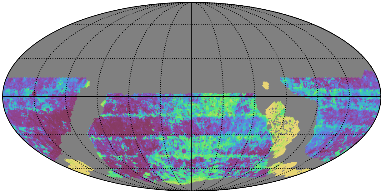
too_elab_r16_d2_giz_v3.4_10yrs WFD y band: Median Inter-Night Gap
