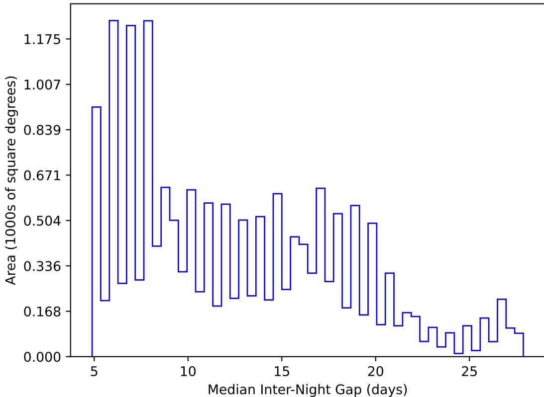
too_elab_r16_d2_giz_v3.4_10yrs WFD y band: Median Inter-Night Gap
