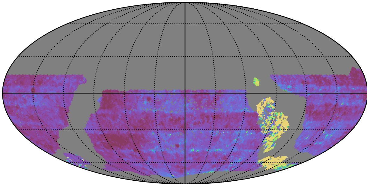
too_elab_r16_d2_giz_v3.4_10yrs WFD u band: Median Inter-Night Gap
