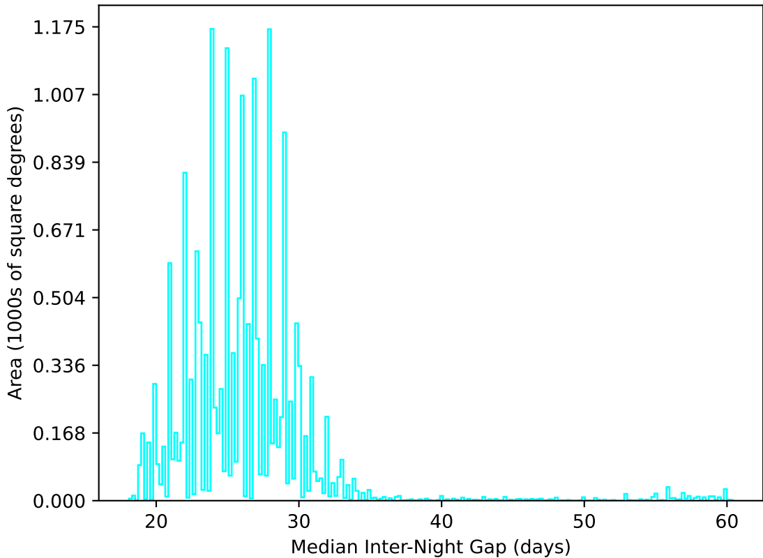
too_elab_r16_d2_giz_v3.4_10yrs WFD u band: Median Inter-Night Gap
