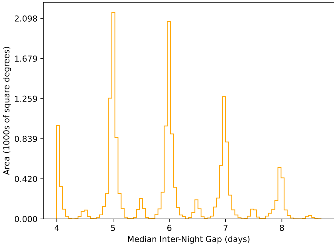
too_elab_r16_d2_giz_v3.4_10yrs WFD r band: Median Inter-Night Gap
