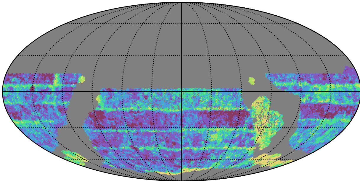
too_elab_r16_d2_giz_v3.4_10yrs WFD i band: Median Inter-Night Gap
